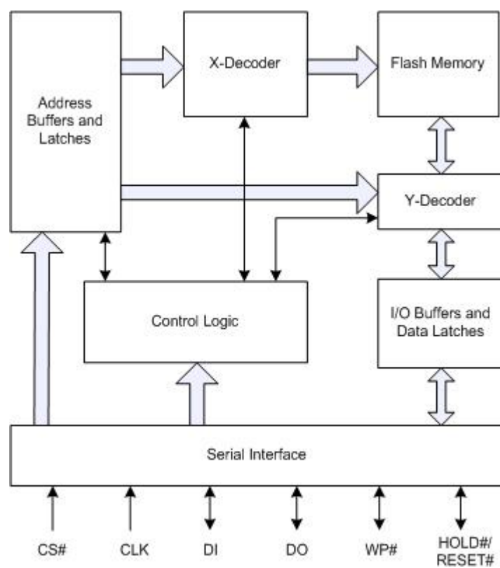
Figure 2.1 Block Diagram
