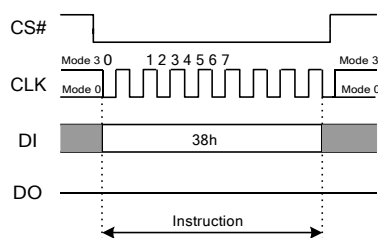
Figure 7.40 Enter QPI Instruction (SPI Mode only)
