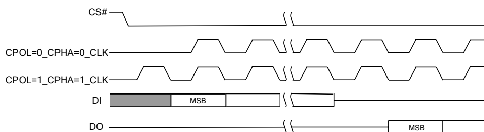
Figure 6.1 SPI Modes
