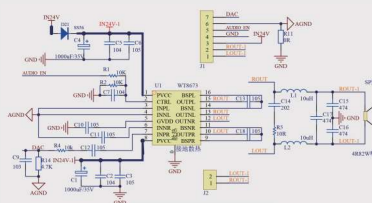
WT8673 application scheme diagram
